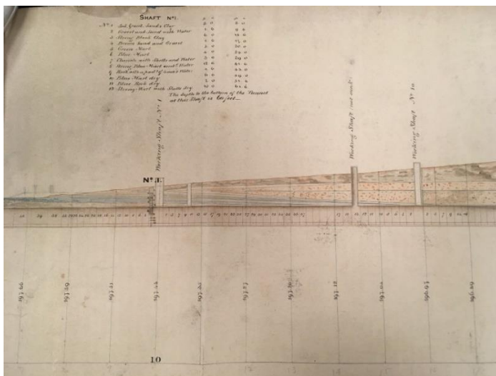
Part of the longitudinal section showing working shafts 1 and 1a
