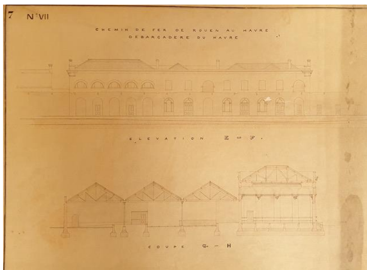
Design for Rouen - Le Havre railway station [ICE Archive]
