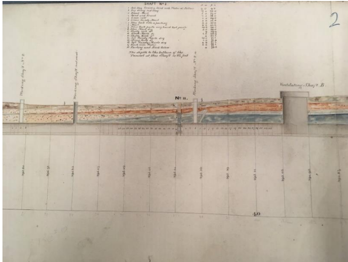
Working shafts 2 and 2a with ventilation shaft B
